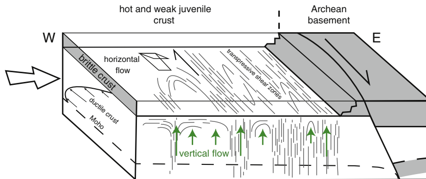
Fig. 13. 3D diagram modified after Gapais et al., 2008. Deformation of a hot and mid-crustal section (Pointe Géologie) in response to a W–E transpressional tectonics. White arrow indicates the horizontal flow marked by mineral stretching lineation in the gneisses. Green arrows indicate the vertical flow point out by AMS analyses only in granitic dykes and anatexites.
