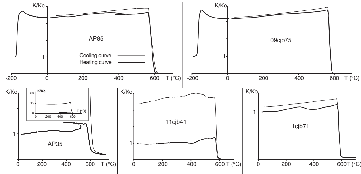
Fig. 6. Normalized susceptibility K/K_o as a function of the temperature T in gneisses (samples AP35 and AP85) and in granites (09cjb75, 11cjb41 and 11cjb71).
