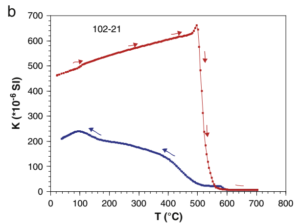
Fig. 7. Thermomagnetic determination of magnetic susceptibility ( K ) versus temperature ( T ) for two samples taken a) at 26 cm from the upper sill margin (sample 102-32), and b) 57 cm from the upper sill margin (sample 102-21) obtained in argon atmosphere. The red curve represents the heating path; the blue curve represents the cooling path. (For interpretation of the references to color in this figure legend, the reader is referred to the web version of this article.)
