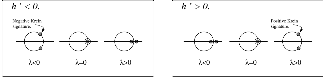
Figure 1. Position of the two critical eigenvalues of \mathbf{M}^\alpha(\lambda) in the case where \lambda is close to 0 and \partial_\lambda \mathbf{C}^\alpha(\cdot, \cdot) is positive.
